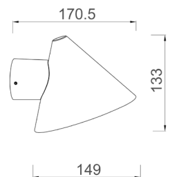
CUCHARA4 (Electroplated Copper Aluminium)
